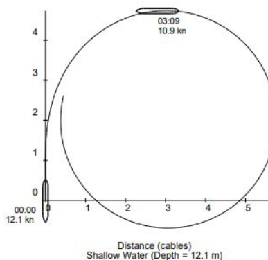
STOPPING CHARACTERISTICS
