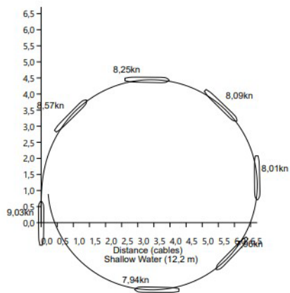
TURNING CIRCLES AT MAX. RUDDER ANGLE (35°)
