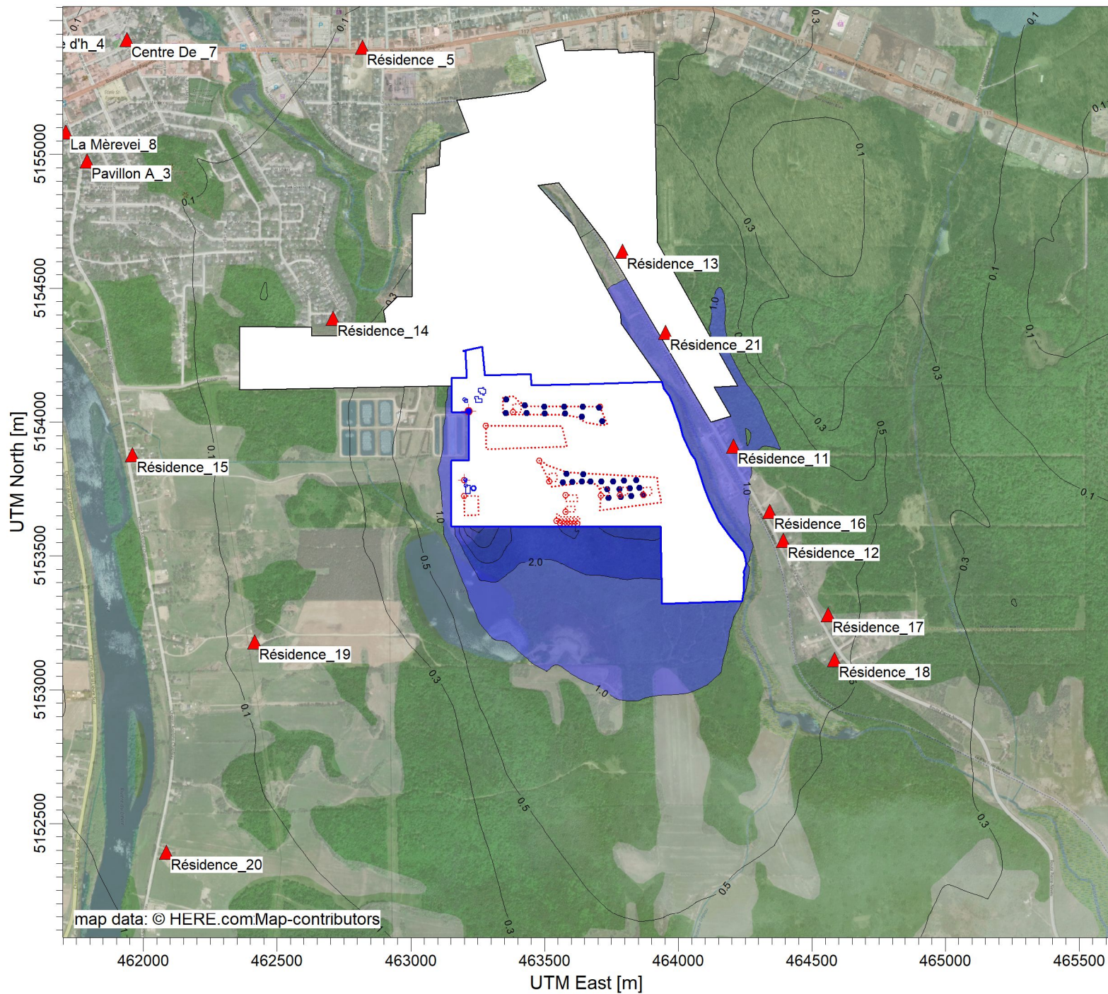
PLOT FILE OF 98.00TH PERCENTILE 4-MIN VALUES FOR SOURCE GROUP: ALL Max: 13.5 [UO/M**3] at (463249.13, 5153609.63)
