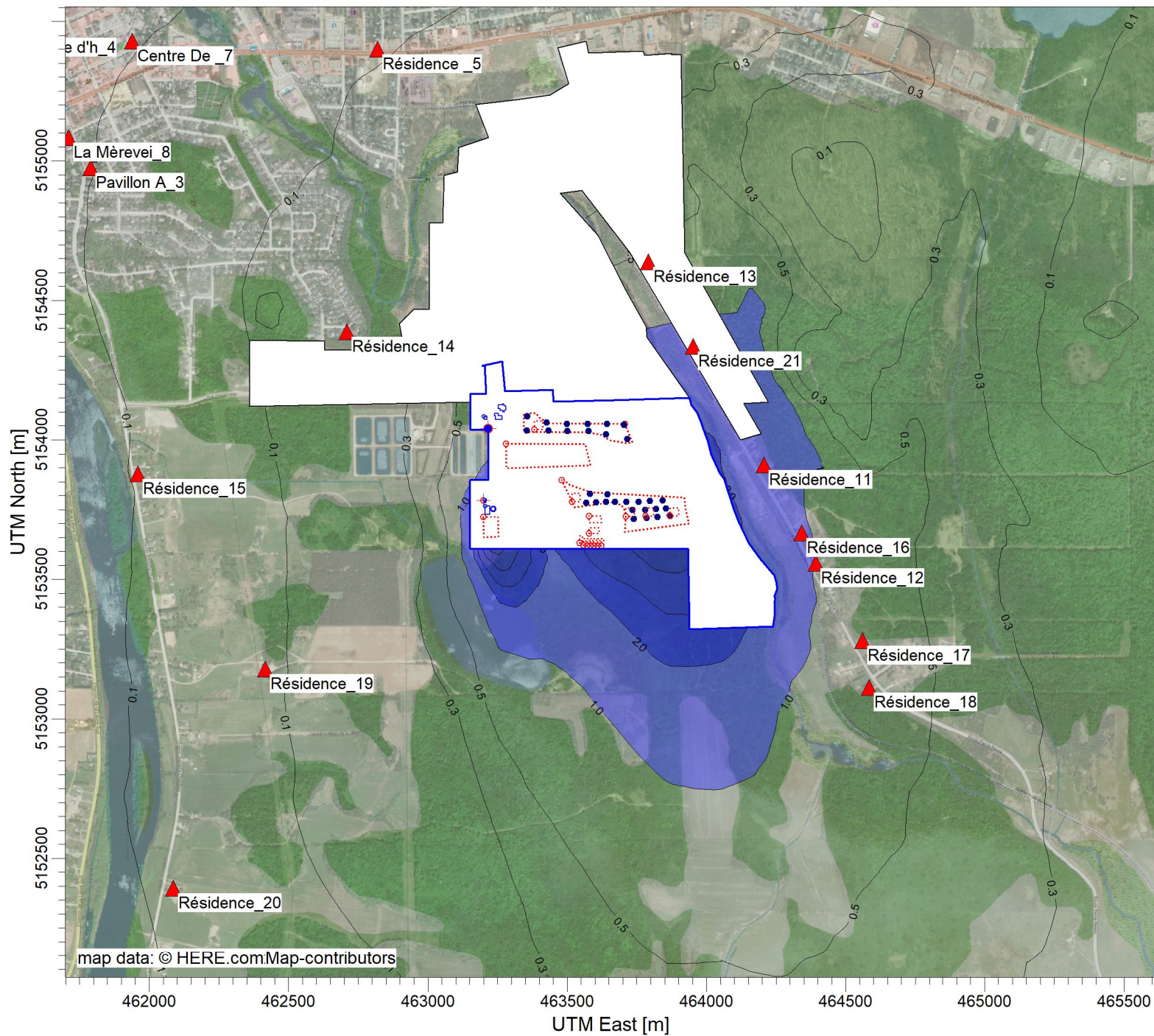
PLOT FILE OF 98.00TH PERCENTILE 4-MIN VALUES FOR SOURCE GROUP: ALL Max: 13.4 [UO/M**3] at (463249.13, 5153609.63)
