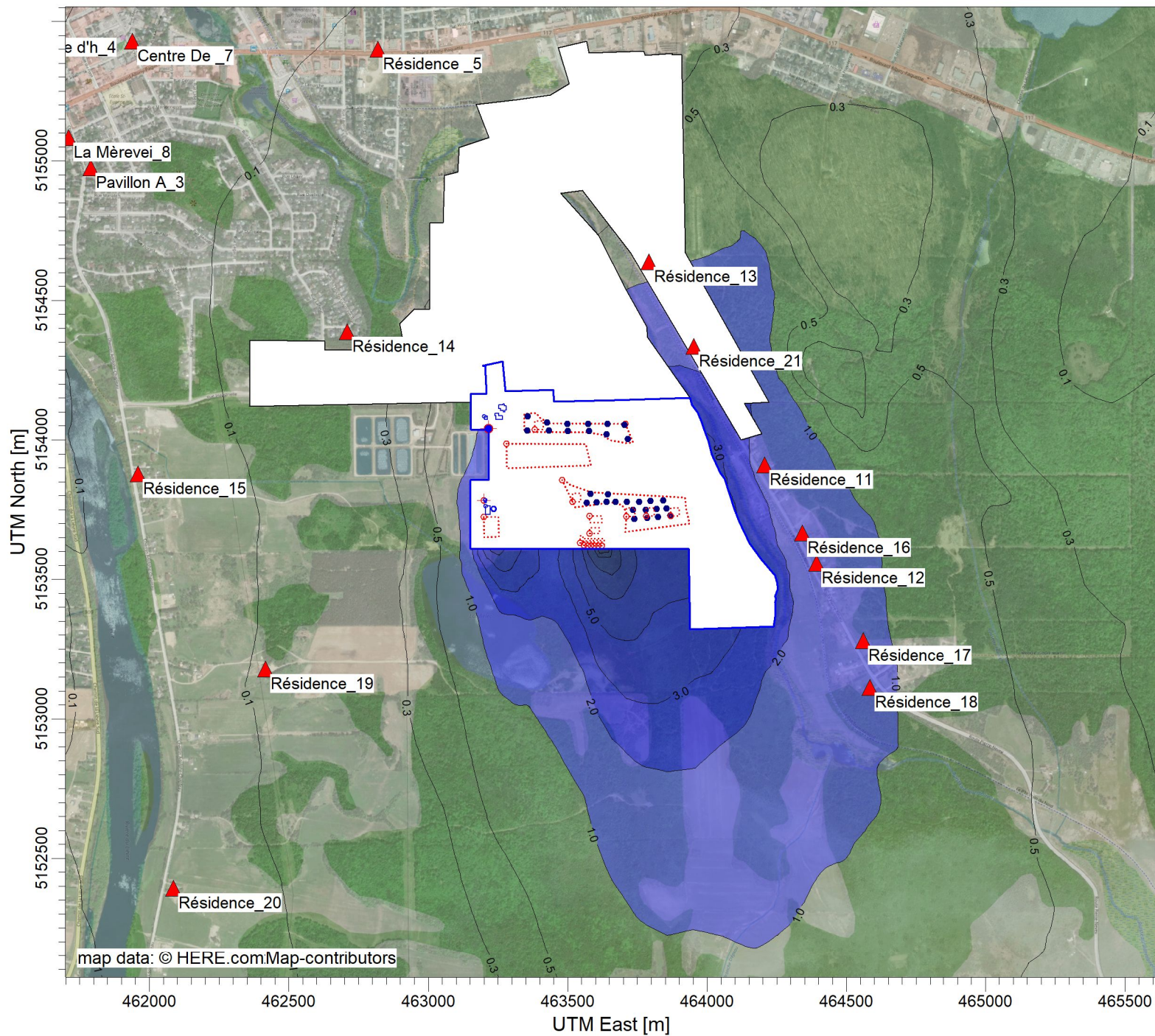
PLOT FILE OF 98.00TH PERCENTILE 4-MIN VALUES FOR SOURCE GROUP: ALL Max: 84.0 [UO/M**3] at (463621.05, 5153608.77) UO/M**3
