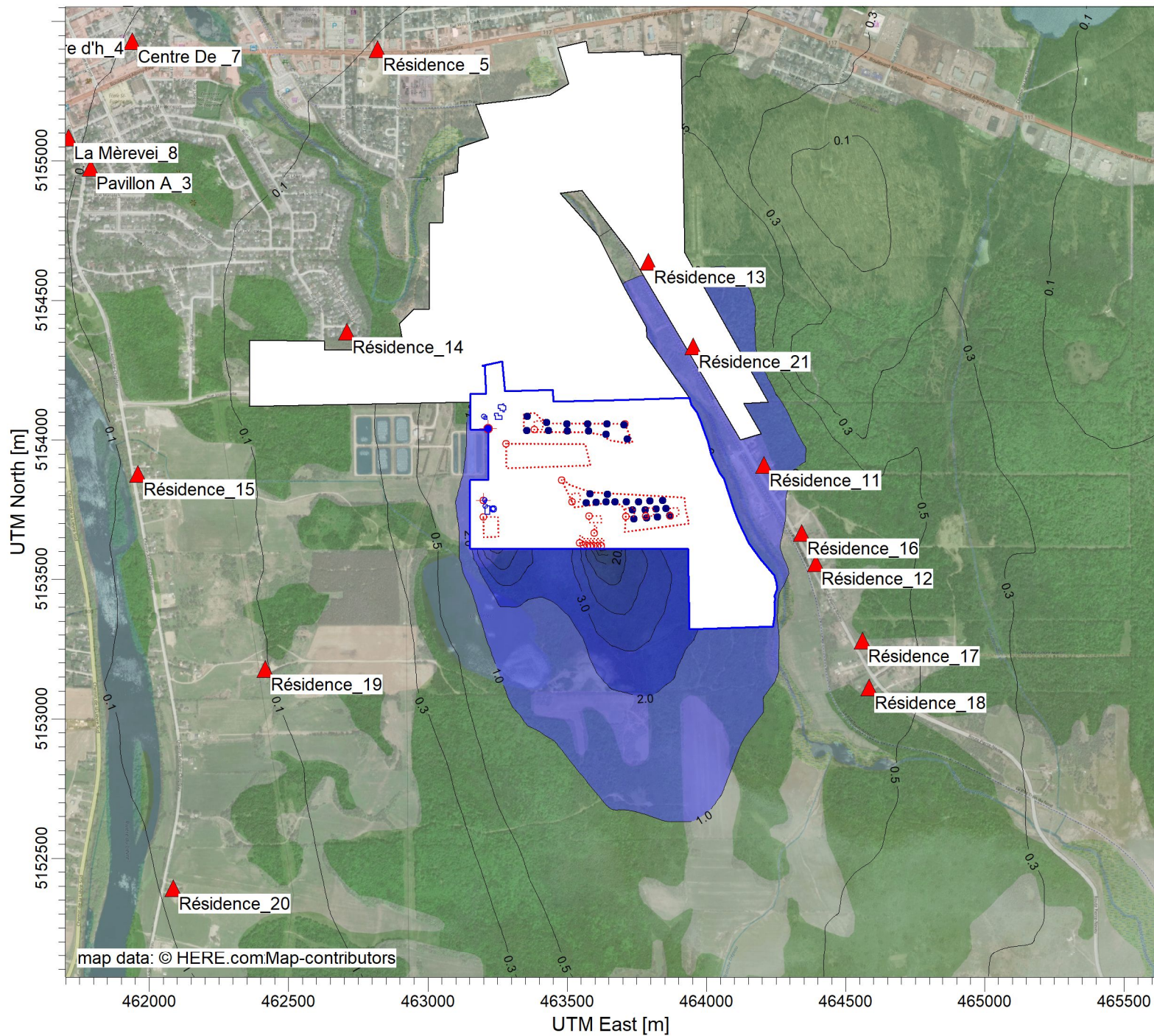
PLOT FILE OF 98.00TH PERCENTILE 4-MIN VALUES FOR SOURCE GROUP: ALL Max: 69.9 [UO/M**3] at (463621.05, 5153608.77)
