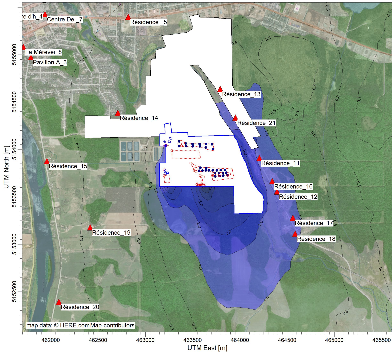
PLOT FILE OF 98.00TH PERCENTILE 4-MIN VALUES FOR SOURCE GROUP: ALL Max: 72.1 [UO/M**3] at (463621.05, 5153608.77)
