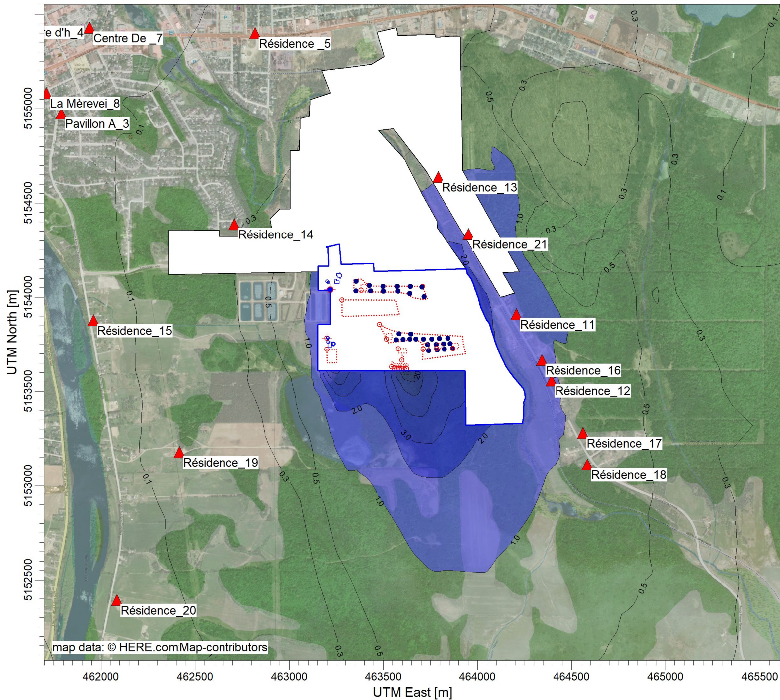
PLOT FILE OF 98.00TH PERCENTILE 4-MIN VALUES FOR SOURCE GROUP: ALL Max: 70.3 [UO/M**3] at (463621.05, 5153608.77)
