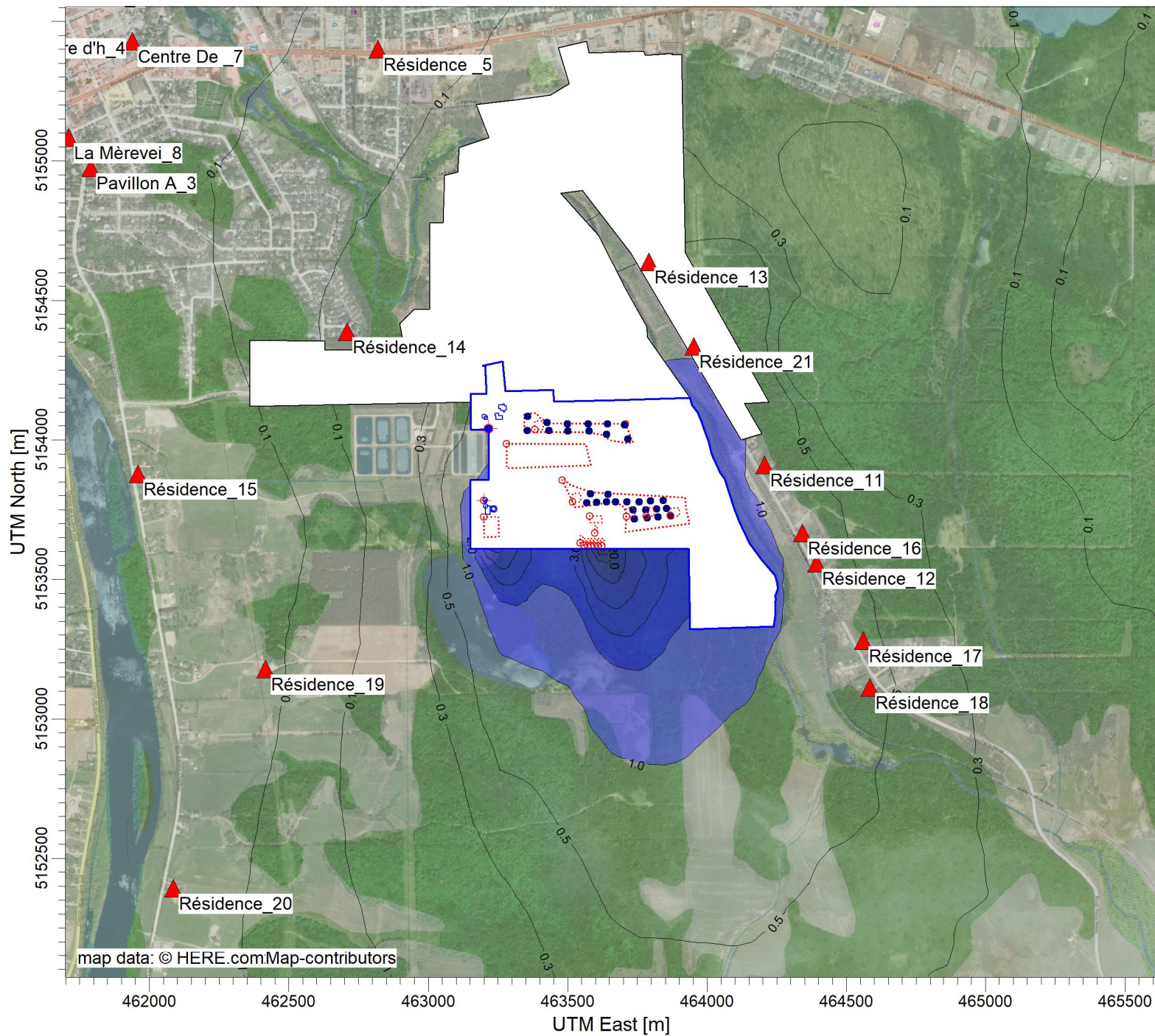
PLOT FILE OF 98.00TH PERCENTILE 4-MIN VALUES FOR SOURCE GROUP: ALL Max: 68.6 [UO/M**3] at (463621.05, 5153608.77)
