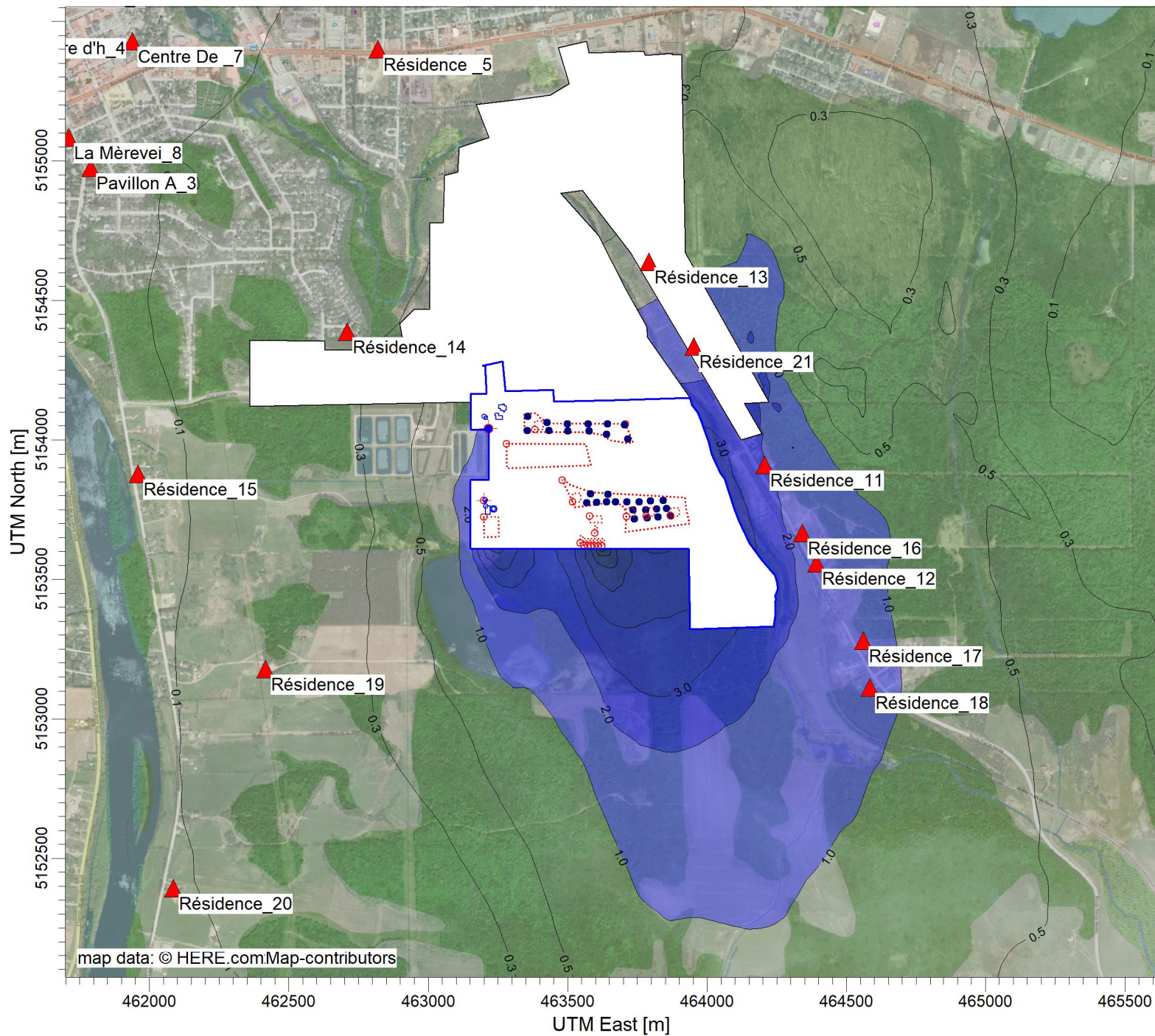
PLOT FILE OF 98.00TH PERCENTILE 4-MIN VALUES FOR SOURCE GROUP: ALL Max: 73.2 [UO/M**3] at (463621.05, 5153608.77)
