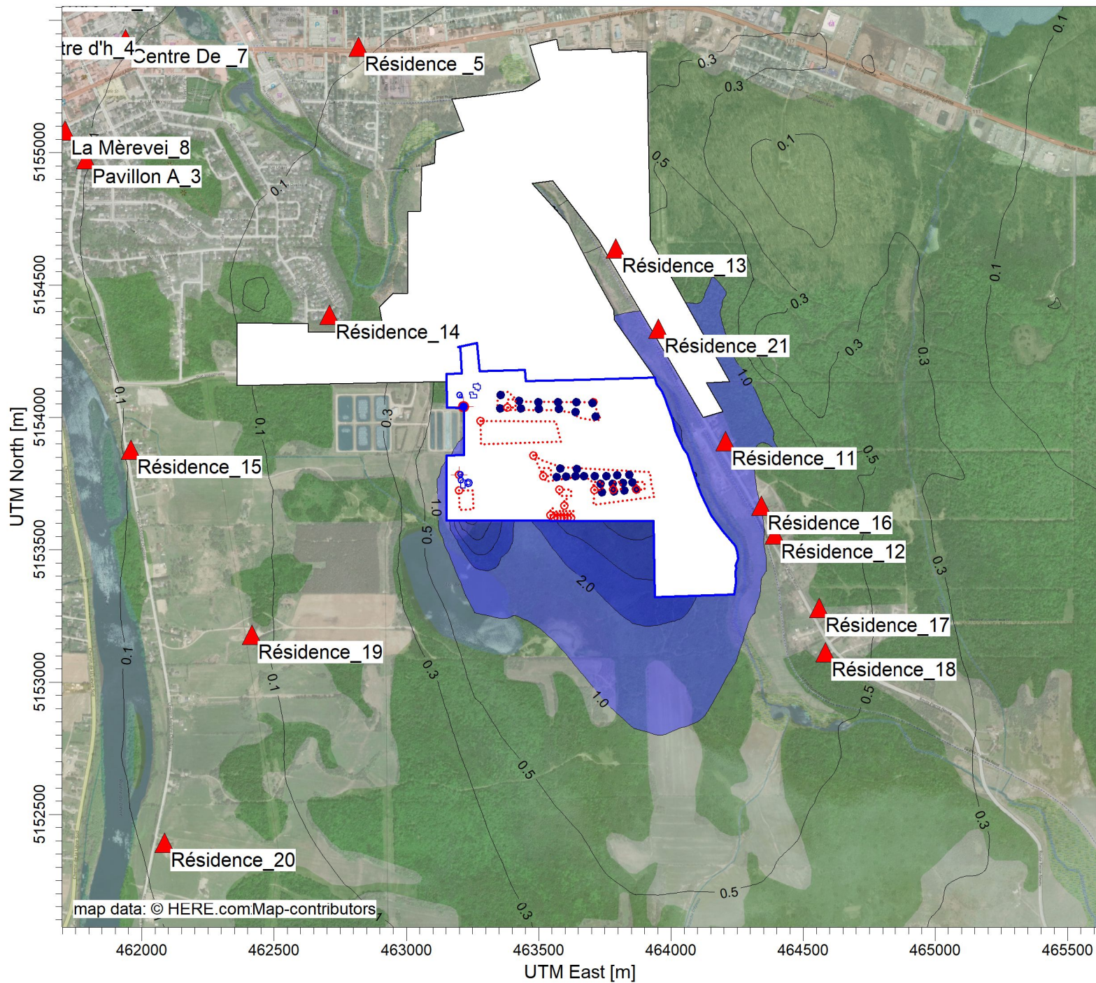
PLOT FILE OF 98.00TH PERCENTILE 4-MIN VALUES FOR SOURCE GROUP: ALL Max: 12.0 [UO/M**3] at (463249.13, 5153609.63)
