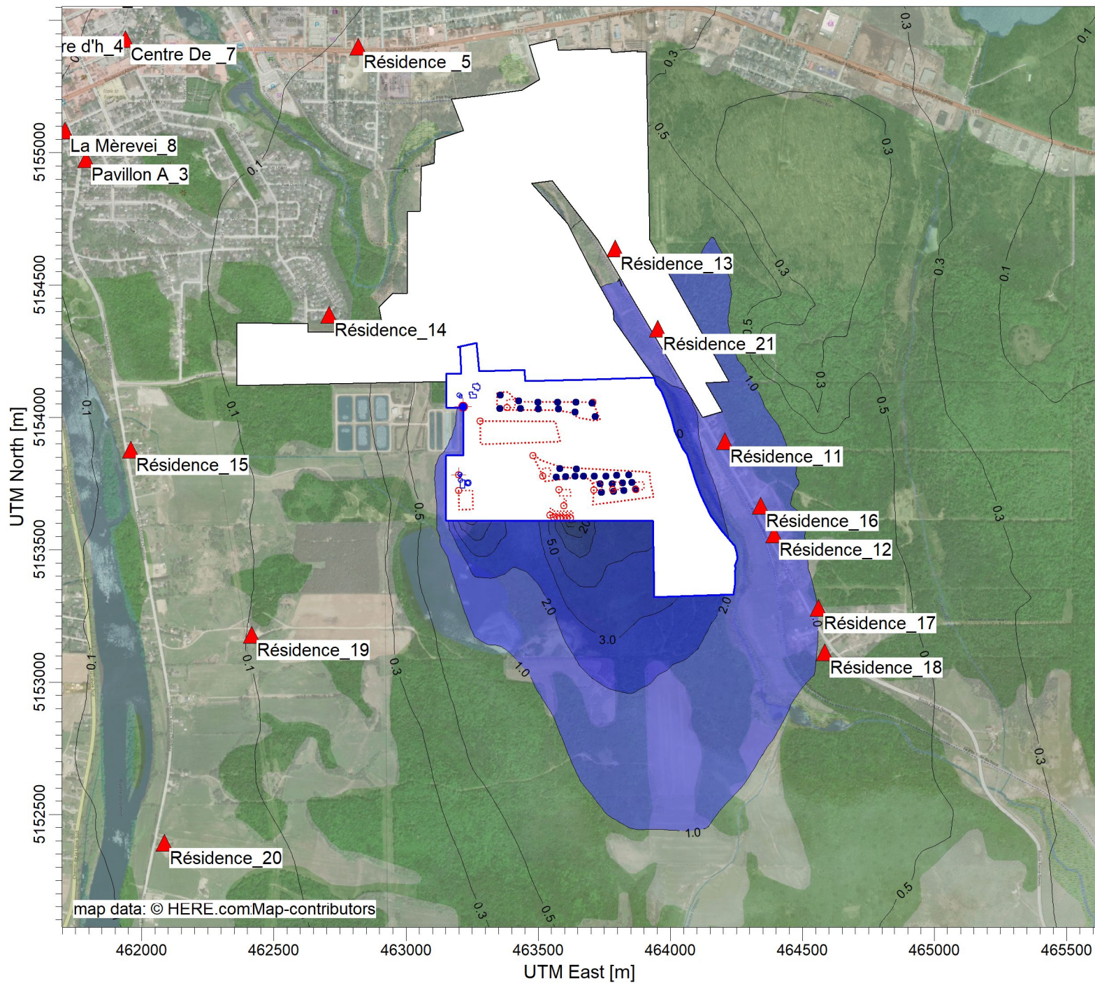
PLOT FILE OF 98.00TH PERCENTILE 4-MIN VALUES FOR SOURCE GROUP: ALL Max: 71.2 [UO/M**3] at (463621.05, 5153608.77)
