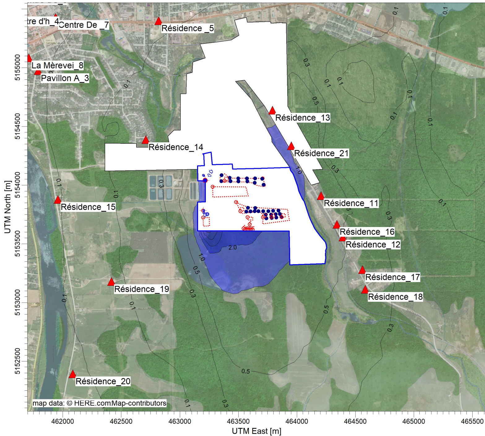
PLOT FILE OF 98.00TH PERCENTILE 4-MIN VALUES FOR SOURCE GROUP: ALL Max: 12.1 [UO/M**3] at (463249.13, 5153609.63)
