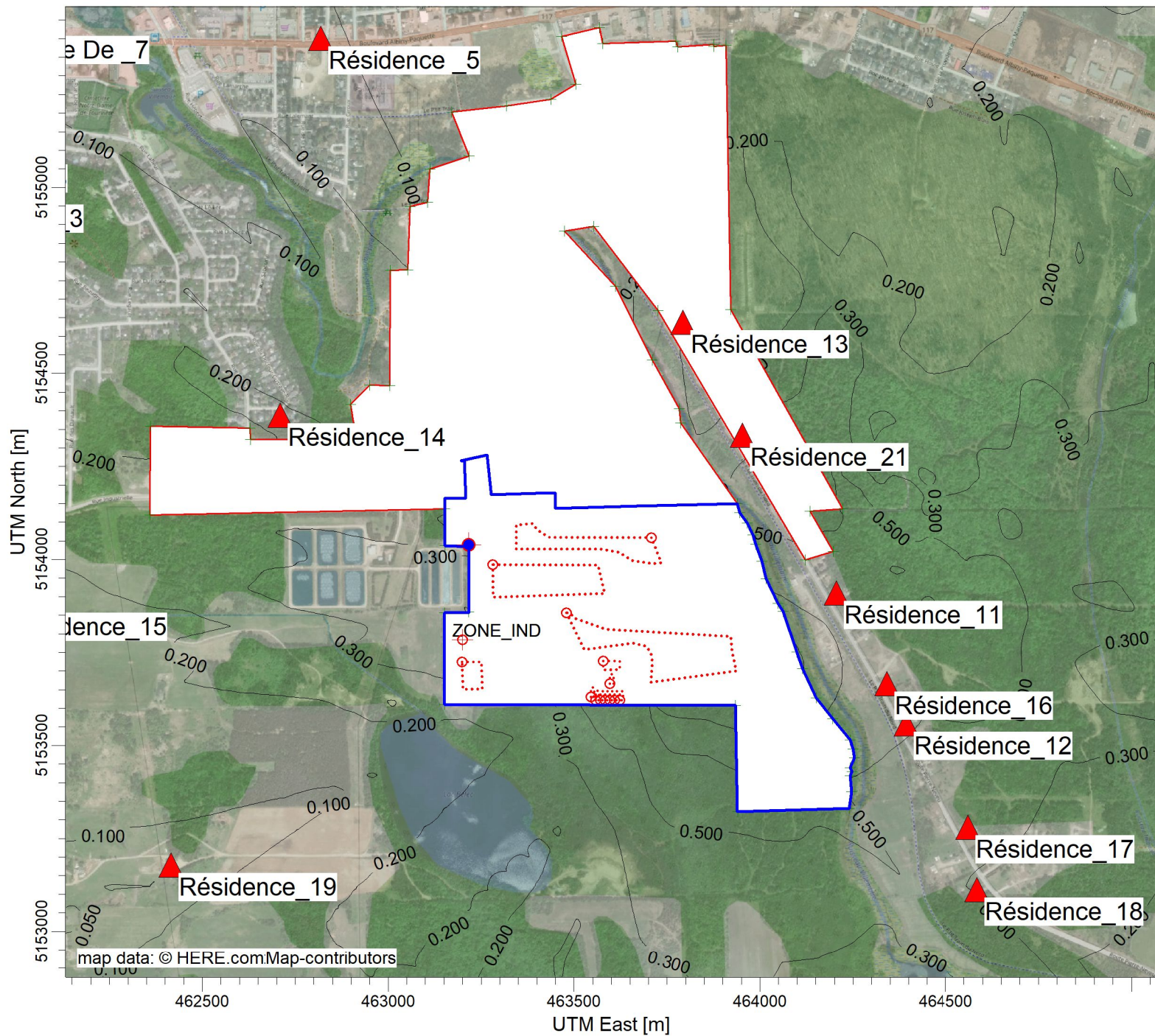
PLOT FILE OF HIGH 1ST HIGH 1-HR VALUES FOR SOURCE GROUP: ALL Max: 1.170 [ug/m^3] at (463875.53, 5153608.18) ug/m^3
