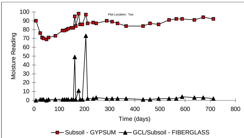
Figure D.5: MOISTURE READINGS VS. TIME FOR PLOT E (Gundseal - Bentonite Side Down - 3:1 Slope)
