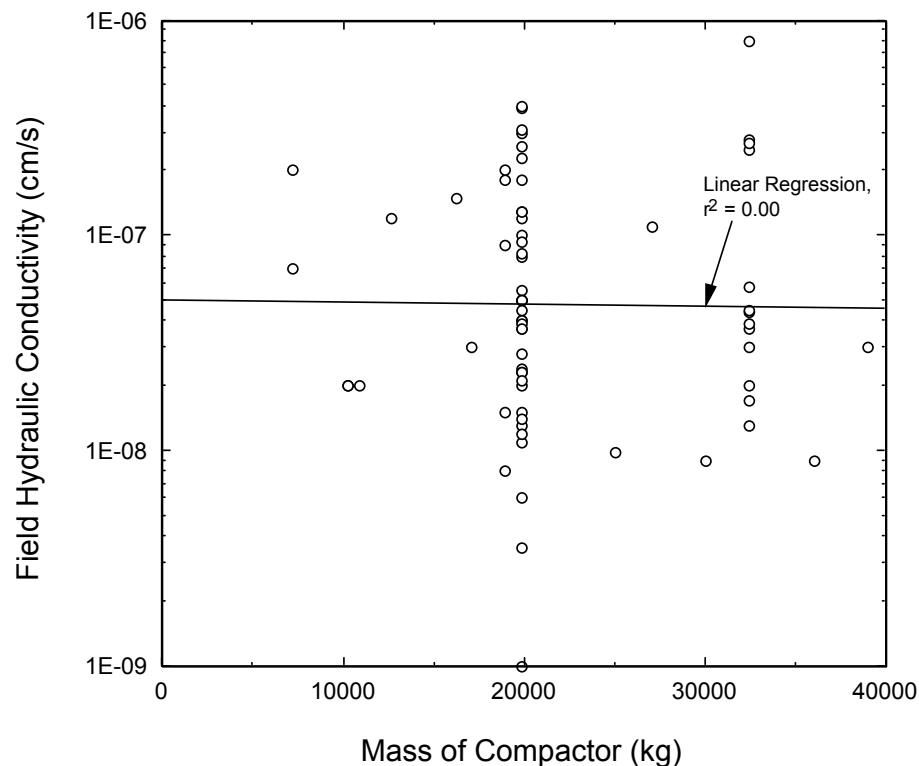
Figure 4-27. Field hydraulic conductivity versus mass of compactor.
