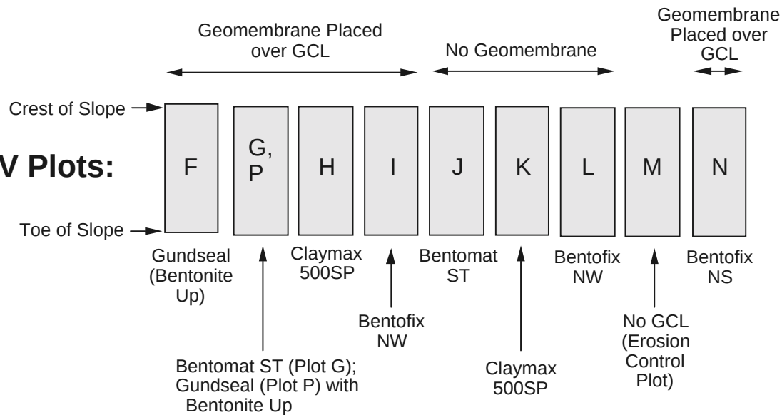
Figure D-1. Layout of field test plots.
