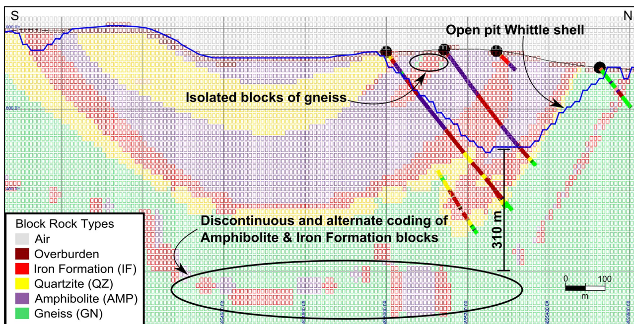
Figure 14–14: Cross-Section 614425 Illustrating Minor Issues in Codification of Rock Type Model
