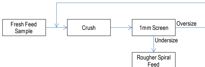
Figure 13-2: Sample Preparation (crushing and screening) Testwork Flow Diagram
