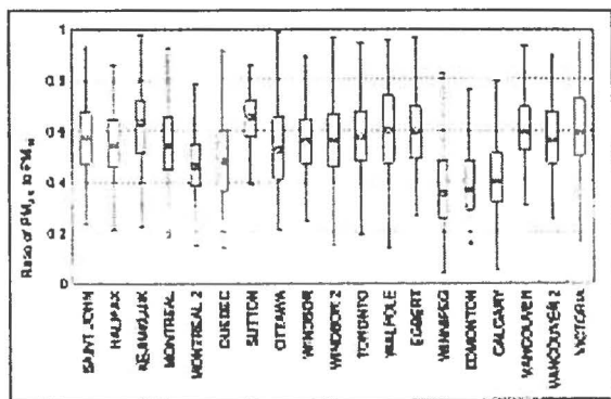
FIGURE 2 Distributions of the ratio of PM 2.5 to PM 10 mass at the NAPS dichotomous sampler sites. The box plots indicate the median, 5th and 95th and 25th and 75th percentiles (from Brook et al. , 1997).
