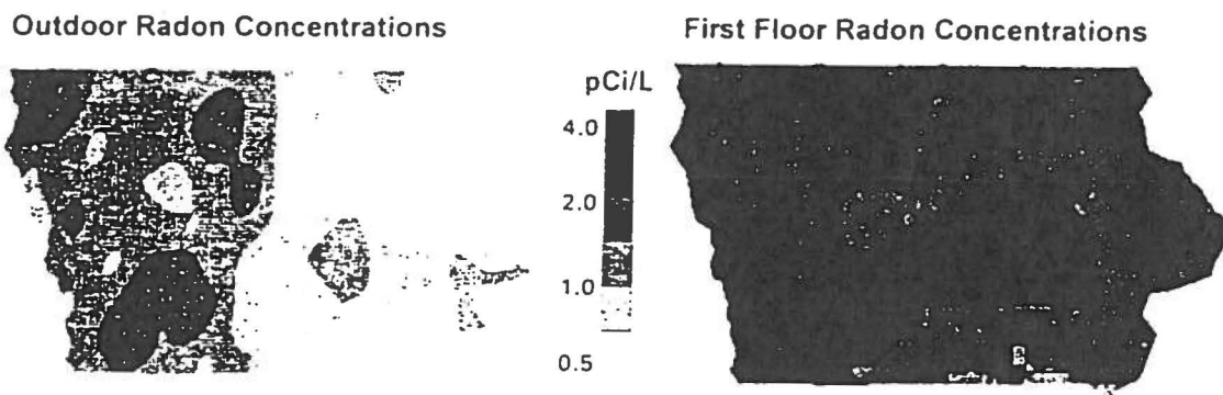
FIGURE 1. Maps of outdoor and first-floor radon concentrations in Iowa, IRLCS, 1993–1997.
